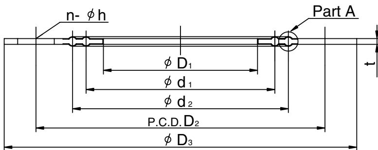
PTFE-Covering
