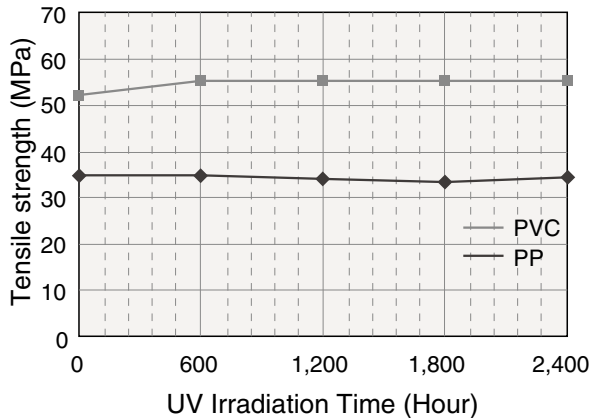
- Acceleration Test Data by Sunshine Weather Meter -
